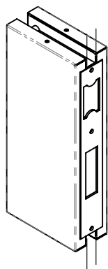
Controcartella verticale Vertical strike box Cerradero vertical
